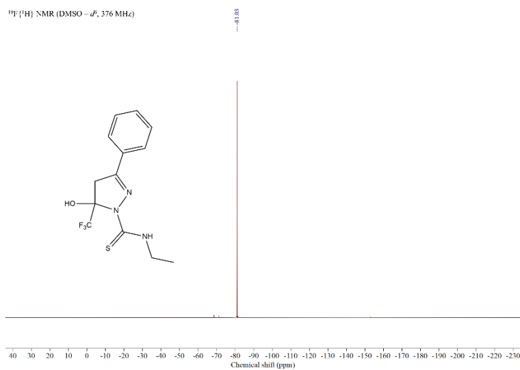
Figure S9. 19 F{ 1 H} NMR spectrum of thiosemicarbazone 3 , in DMSO – d 6 solution.
