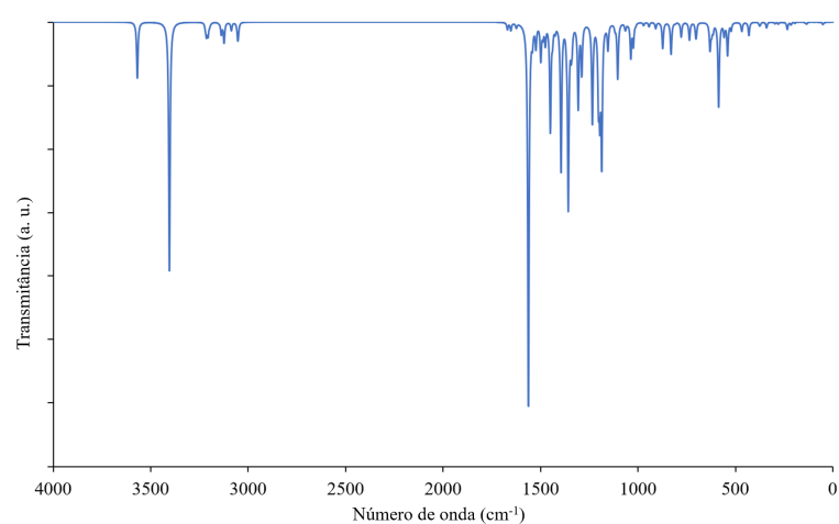
Figure S15. Calculated IR spectrum on thiosemicarbazone 3.
