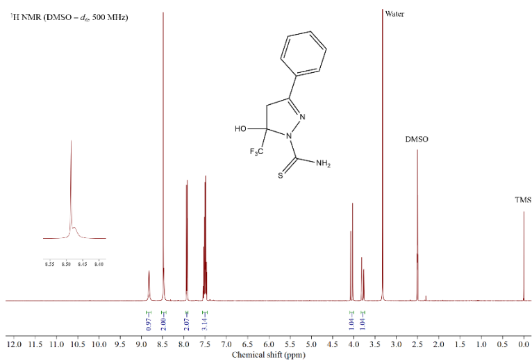
Figure S4. ^1\text{H} NMR spectrum of thiosemicarbazone 1 , in \text{DMSO}-d_6 solution.
