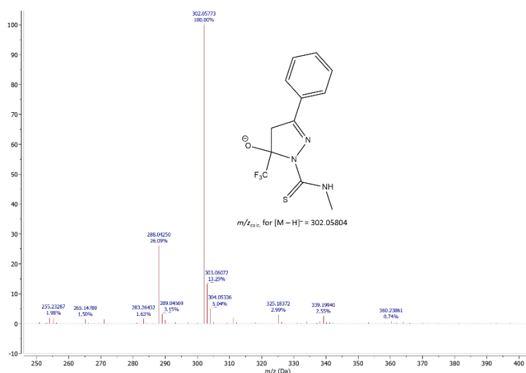
Figure S11. Negative mode mass spectrum of thiosemicarbazone 2 , in acetonitrile solution.
