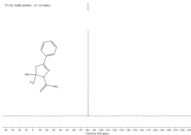
Figure S7. 19 F{ 1 H} NMR spectrum of thiosemicarbazone 1 , in DMSO – d 6 solution.
