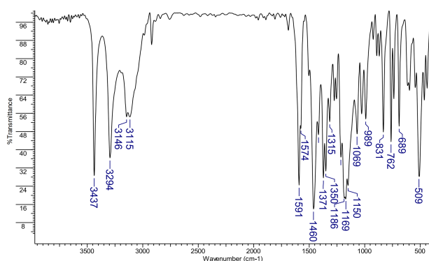
Figure S1. Infrared spectrum of thiosemicarbazone 1 .
