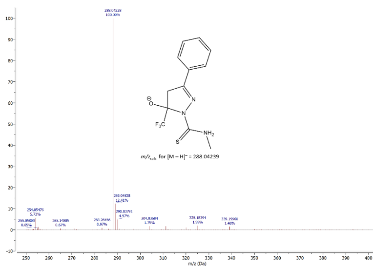
Figure S10. Negative mode mass spectrum of thiosemicarbazone 1 , in acetonitrile solution.
