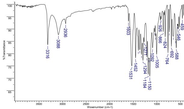
Figure S2. Infrared spectrum of thiosemicarbazone 2 .
