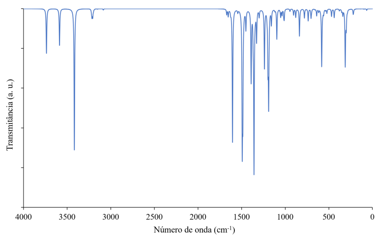
Figure S13. Calculated IR spectrum on thiosemicarbazone 1.
