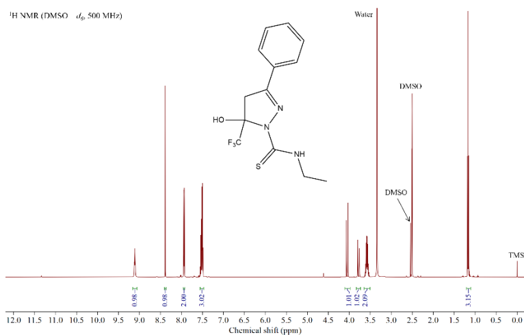
Figure S6. ^1\text{H} NMR spectrum of thiosemicarbazone 3 , in DMSO - d_6 solution.
