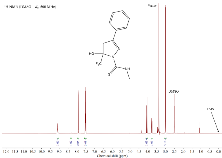
Figure S5. ^1\text{H} NMR spectrum of thiosemicarbazone 2 , in DMSO - d_6 solution.
