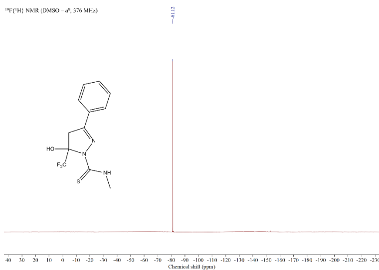
Figure S8. 19 F{ 1 H} NMR spectrum of thiosemicarbazone 2 , in DMSO – d 6 solution.
