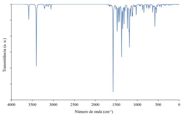
Figure S14. Calculated IR spectrum on thiosemicarbazone 2.
