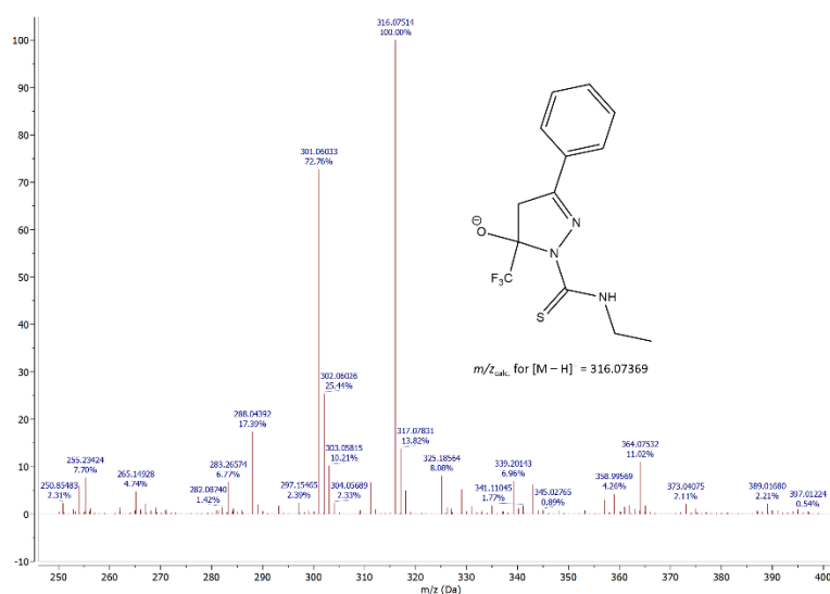
Figure S12. Negative mode mass spectrum of thiosemicarbazone 3 , in acetonitrile solution.
