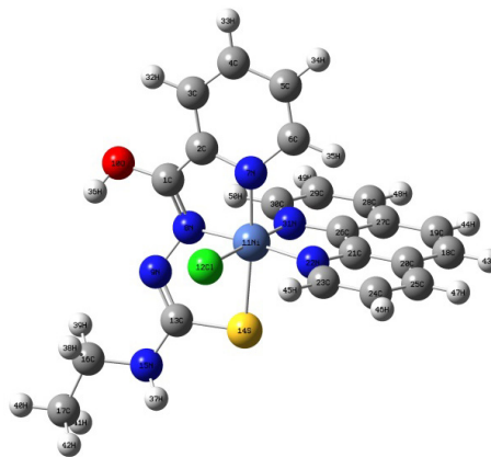
Figure 4. The optimized structural geometry of [Ni(EPHC)(1,10-phen)Cl] (2) along with the atom numbering scheme.
